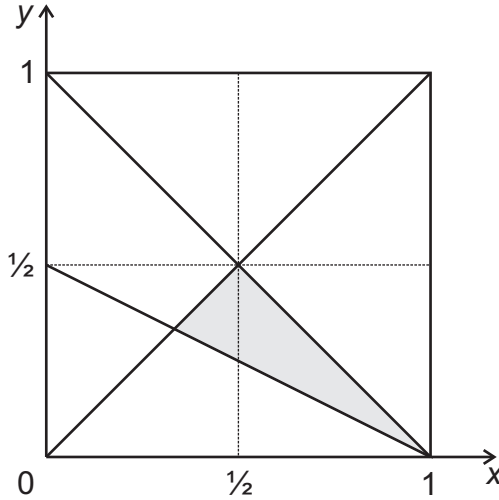
Figure 1. Shaded triangle contains all three-candidate elections in which the vote fractions of candidates A, B, and C are x, y, and z = 1 - x - y.
