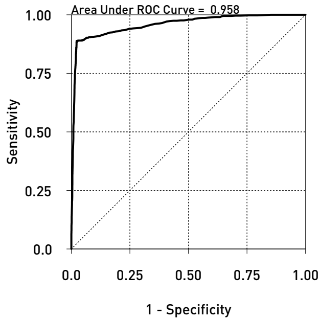
Figure 4: ROC Curves for Ordinary Probit and Transition Models
