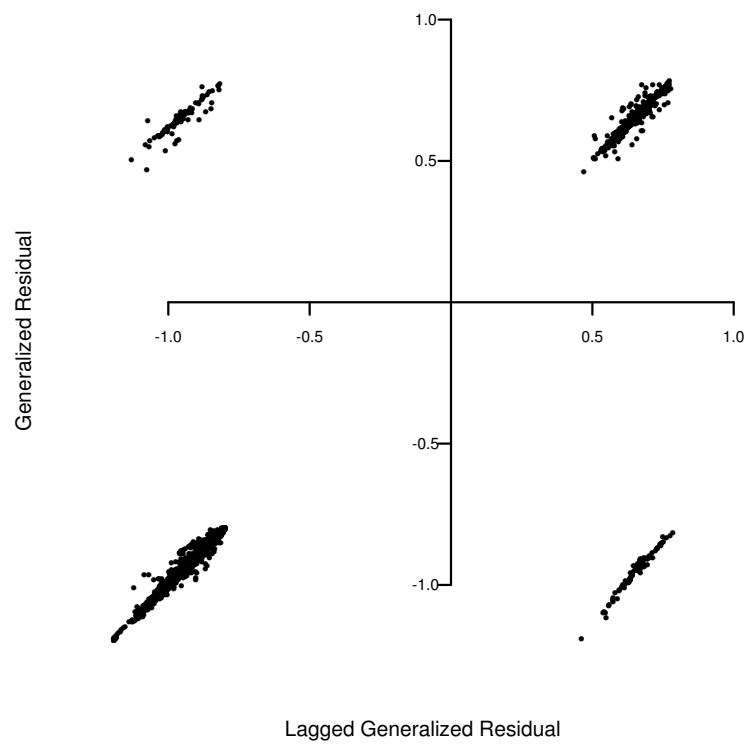
Figure 3: Residuals vs Lagged Residuals, Ordinary Probit
